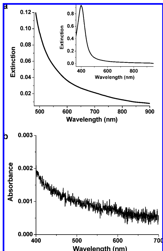
Figure 4. (a) Expanded extinction spectrum of a silver nanoparticle solution prior to irradiation. The inset is the full spectrum. (b) UV-vis spectrum of a mixture of \text{AgNO}_3 , citrate, and BSPP. Each reagent is 1 mM.
