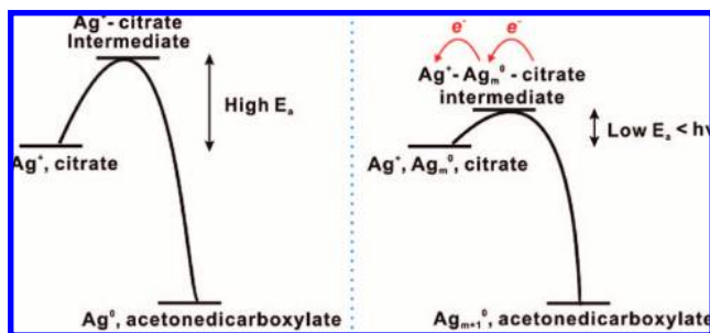
Figure 5. Scheme showing the activation energy for the reaction between \text{Ag}^+ and citrate, and the proposed effect of silver nanoparticles upon photoexcitation.
