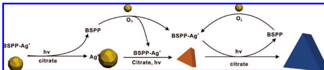
Scheme 3. Proposed Photomediated Growth Pathway of Silver Nanoprisms from Spherical Nanoparticles
