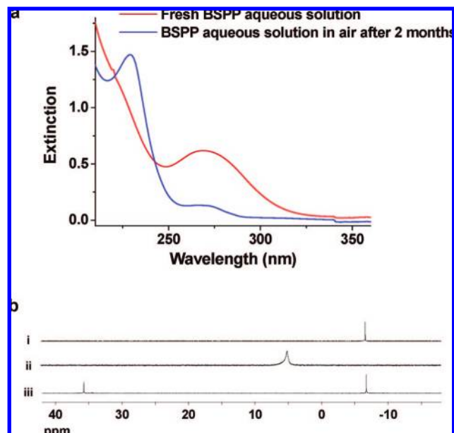
Figure 3. (a) UV-vis spectrum of a 0.05 mM BSPP solution at time 0 and after 2 months in air. (b) ^{31}\text{P} NMR spectra of (i) BSPP, \delta -6.49 ppm; (ii) BSPP:Ag ^{+} = 5:1, \delta 5.05 ppm; and (iii) BSPP and BSPP=O, \delta -6.49 , 36.40 ppm.
