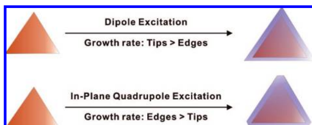
Scheme 4. Triangular Prisms with Sharp Tips Form from Dipole Excitation because Tip Growth Is Faster than Edge Growth; Truncated Prisms Form from Quadrupole Excitation because under These Conditions, Edge Growth Is Faster than Tip Growth
