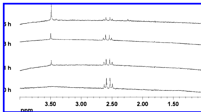
Figure 2. 1 H NMR spectroscopy mapping the fate of citrate during the photochemical prism growth process.
