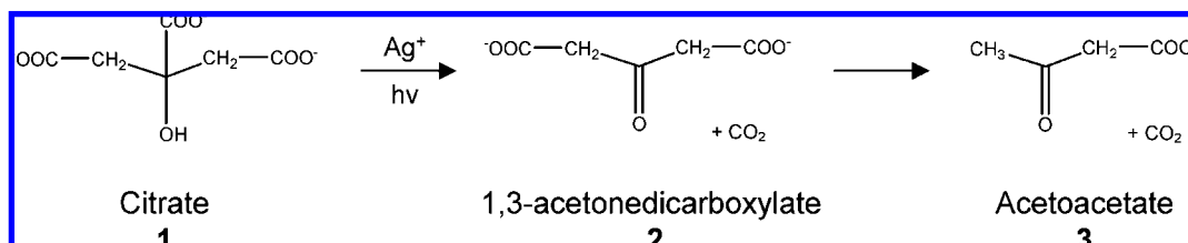
Scheme 1. Degradation Pathway for Citrate during the Photoreaction
