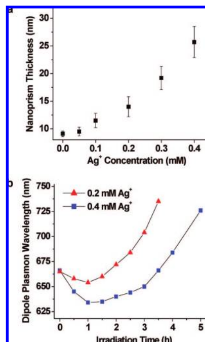
Figure 9. (a) Plot of nanoprisim thickness as a function of \text{Ag}^+ concentration. [0.0] represents the point where no \text{Ag}^+ has been added to the solution. The other points are where the \text{Ag}^+ concentration has been raised through the addition of \text{AgNO}_3 . After irradiation with 550 nm light, the final nanoprisms have an average thickness between 9.1 \pm 0.5 and 25.7 \pm 2.8 nm, depending upon \text{Ag}^+ concentration. (b) Dipole plasmon wavelength of the nanoprisim colloid as a function of irradiation time and \text{Ag}^+ concentration.
