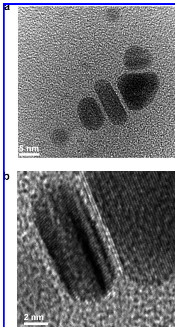
Figure 6. (a) TEM image of the intermediate product, including ellipsoidal particles and a small triangular plate, in the silver colloid after irradiation for 30 min. (b) High-resolution TEM image showing stacking faults in the prisms during growth.
